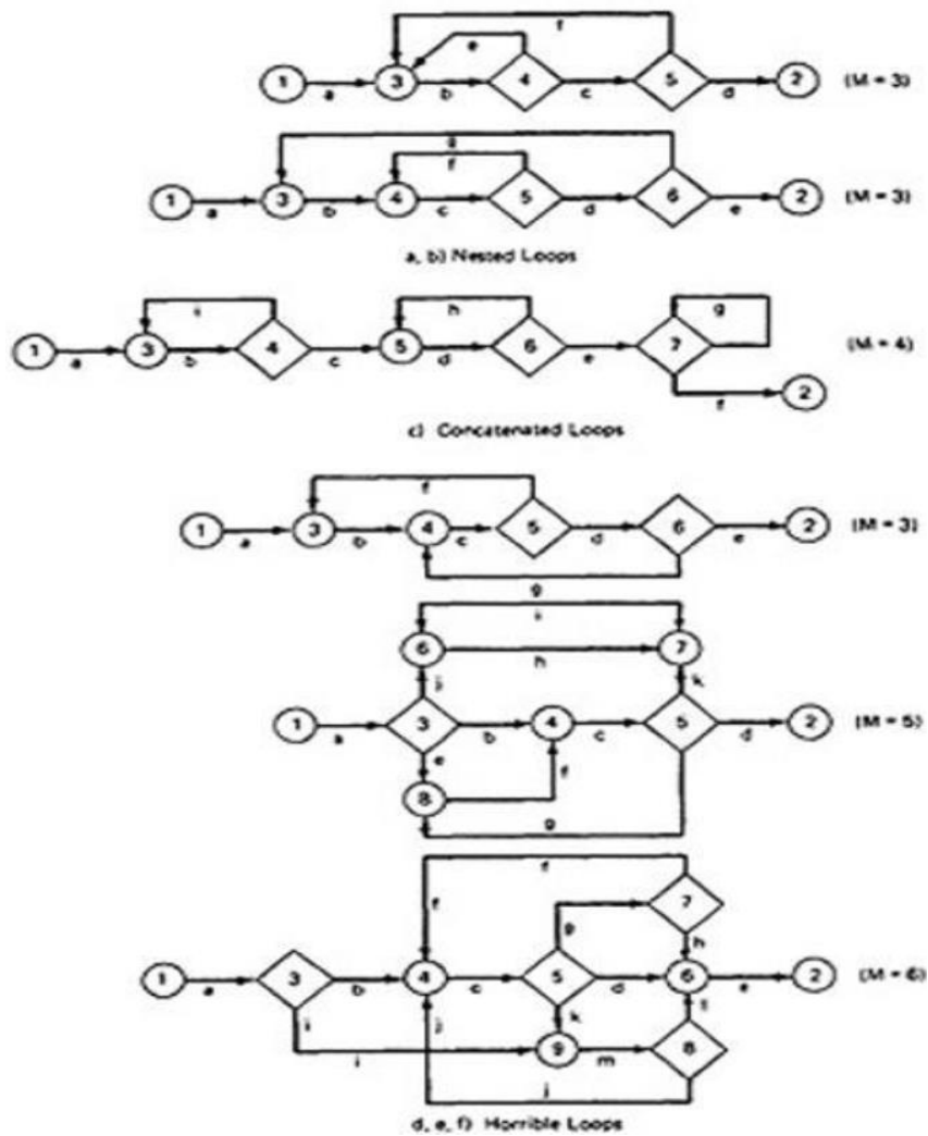
Figure 2.10: Example of Loop types
