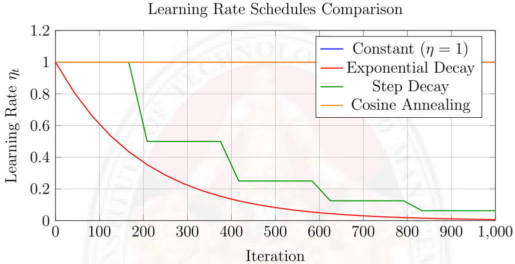
Figure 2.5: Common learning rate schedules for SGD
