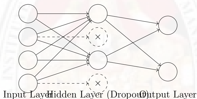
Figure 3.2: Dropout: Randomly dropping neurons during training prevents co-adaptation.
