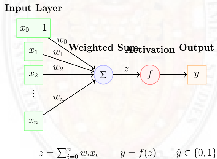
Figure 2.17: Architecture of a Single Perceptron
