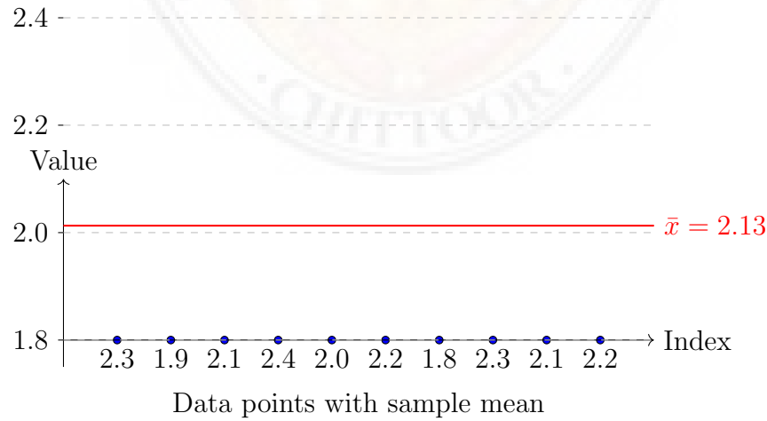
Figure 2.3: Visualization of the 10 data points
