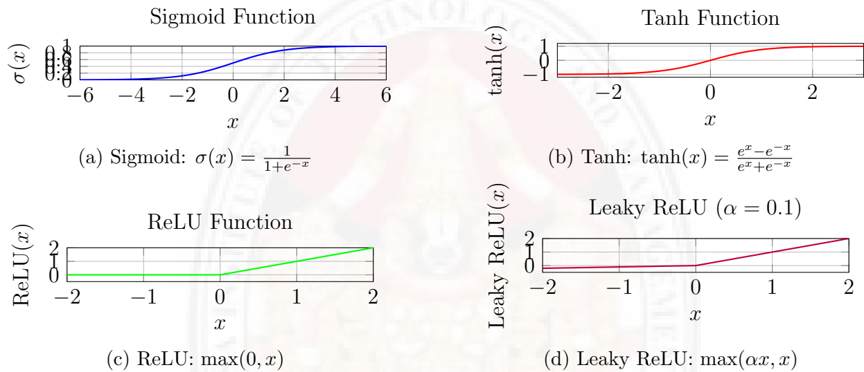
Figure 2.7: Common activation functions with their graphical representations
