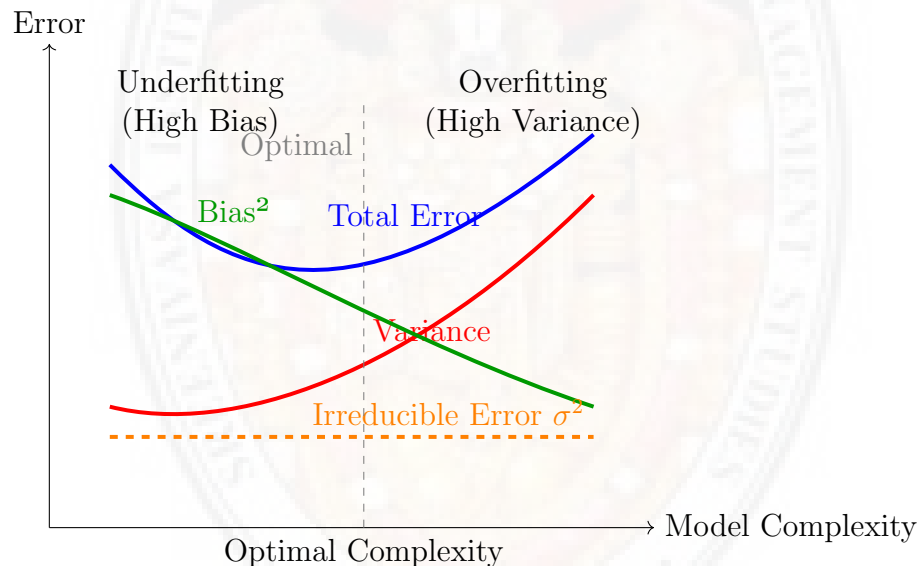
Figure 2.2: Bias-Variance Trade-off: As model complexity increases, bias decreases but variance increases. The optimal model complexity minimizes the total error.
