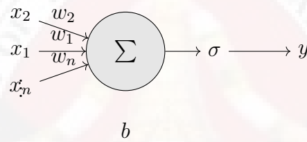
Figure 2.8: McCulloch-Pitts neuron model: y = \sigma(\sum_{i=1}^n w_i x_i + b)
