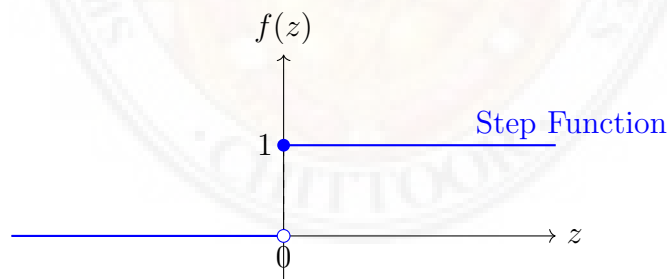
Figure 2.18: Step Activation Function
