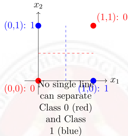
Figure 2.20: XOR Problem - Not Linearly Separable
