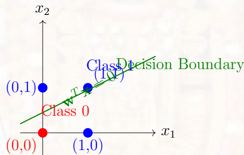
Figure 2.19: Perceptron Decision Boundary for OR Function
