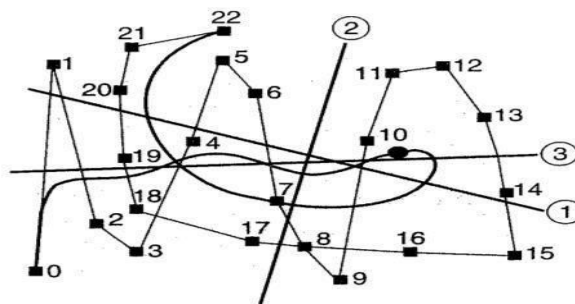
Complexity of characteristic polygon.
