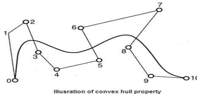
Illustration of convex hull property
