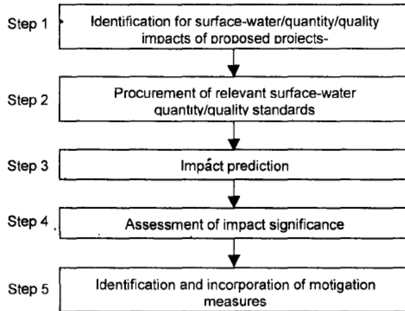
Fig. Conceptual approach to study surface water environment impacts.
