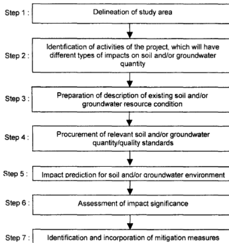
Fig 1: Systematic approach for the study of impacts on soil and ground water.
