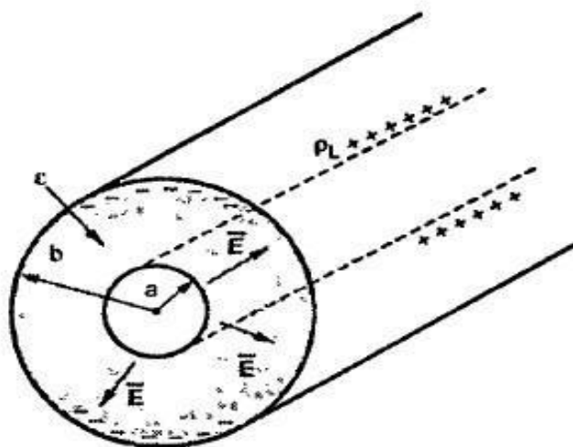
Fig. 5.17 Co-axial cable
