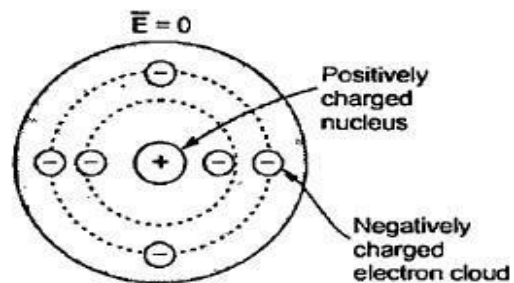
Fig. 5.6 Unpolarized atom of a dielectric
