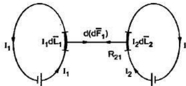
Fig. 8.3 Force between two current elements
