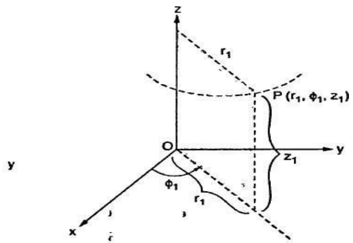
(b) Point P ( r_1, \phi_1, z_1 )
