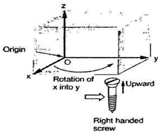
(a) Right handed system
