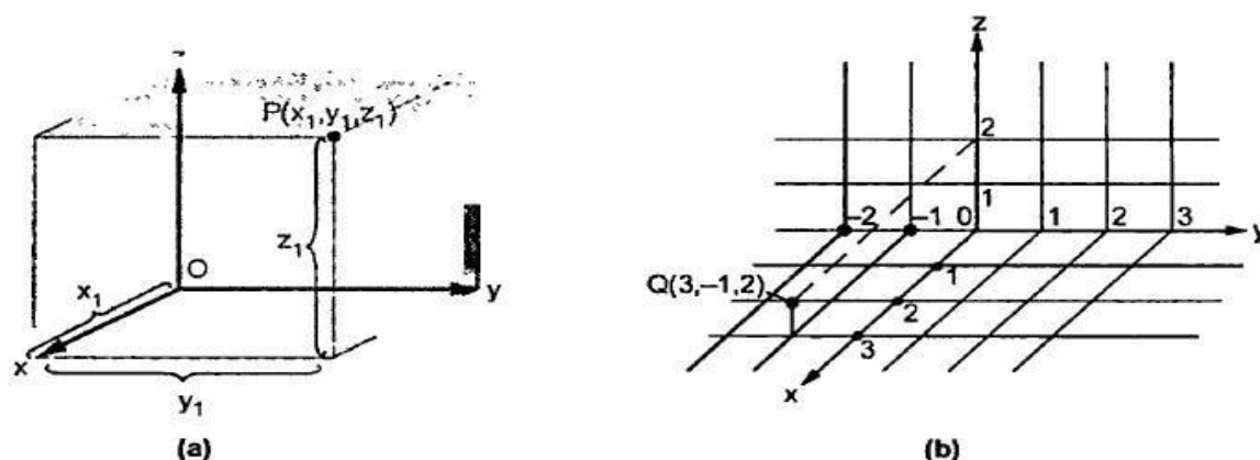
Fig. 1.10 Representing a point in cartesian system
