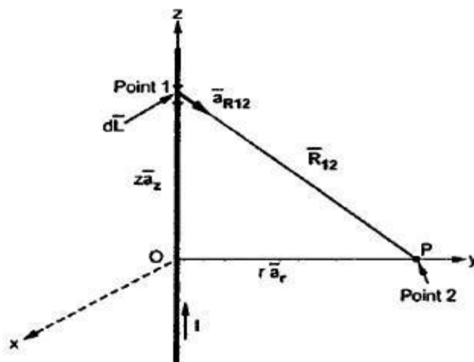
Fig. 7.10 \bar{H} due to infinitely long straight conductor
