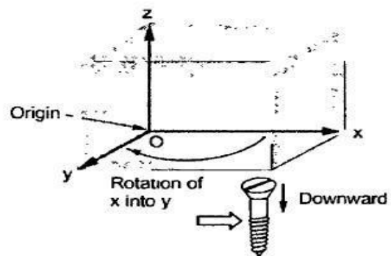
(b) Left handed system
