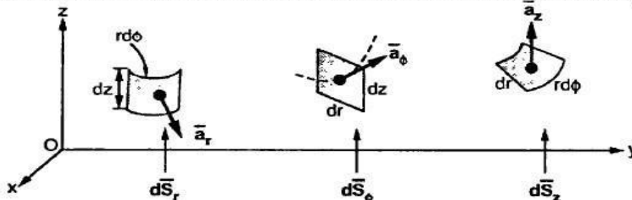
Fig. 1.22 Differential surface elements in cylindrical system
