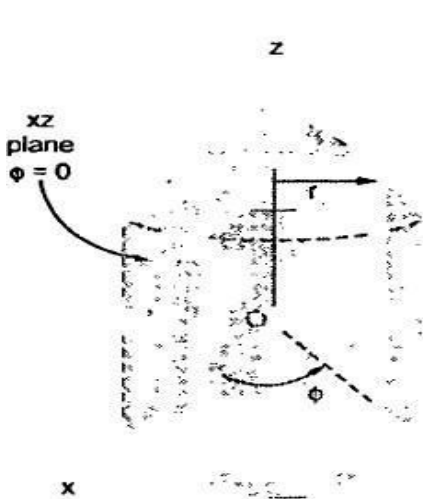
(a) Cylindrical co-ordinate system
