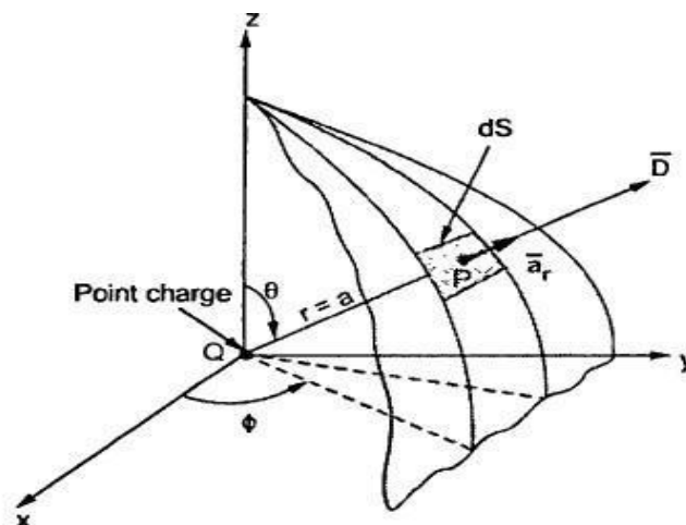
Fig. 3.10 Proof of Gauss's law
