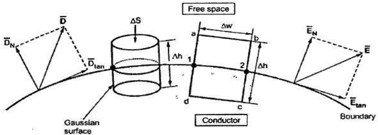
Fig. 5.8 Boundary between conductor and free space
