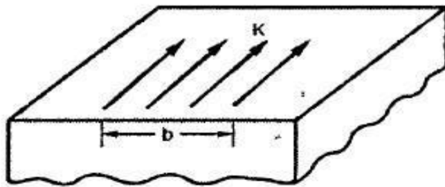
Fig. 7.8 Surface current density
