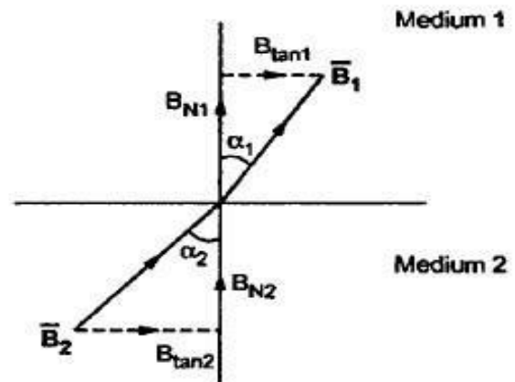
Fig. 8.15 Component of \bar{B} at boundary
