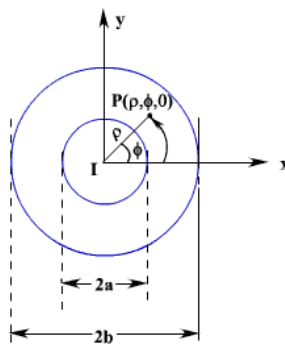
Fig. 4.8: Cross Section of a Coaxial Line
