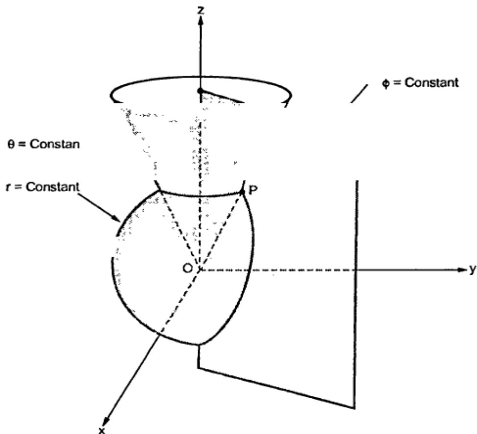
Fig. 1.28 Representing point P in spherical co-ordinate system
