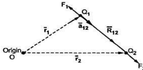
Fig. 2.2 Vector form of Coulomb's law
