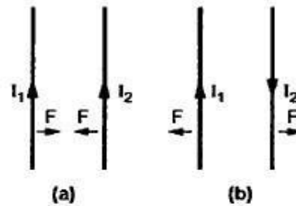
Fig. 8.2 Force between two parallel current carrying conductors
