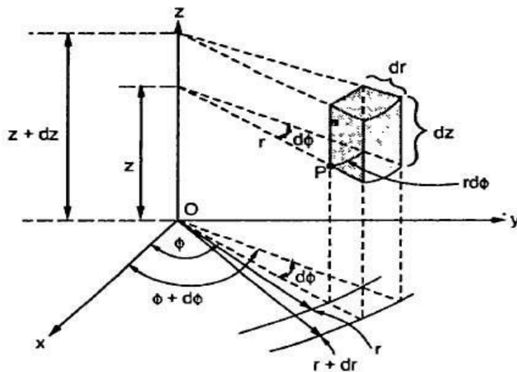
Fig. 1.21 Differential volume in cylindrical co-ordinate system
