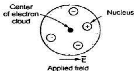
(a) Polarized atom
