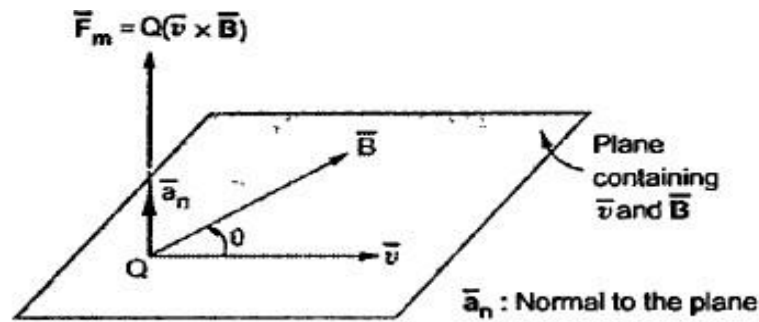
Fig. 8.1 Magnetic force on a moving charge in magnetic field
