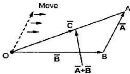
Fig. 1.5 Addition of vectors
