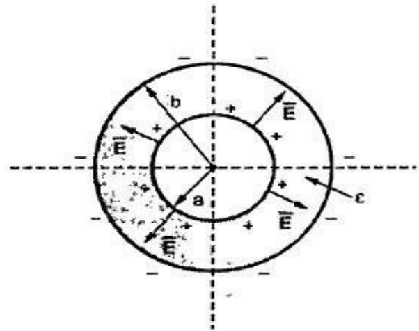
Fig. 5.18 Spherical capacitor
